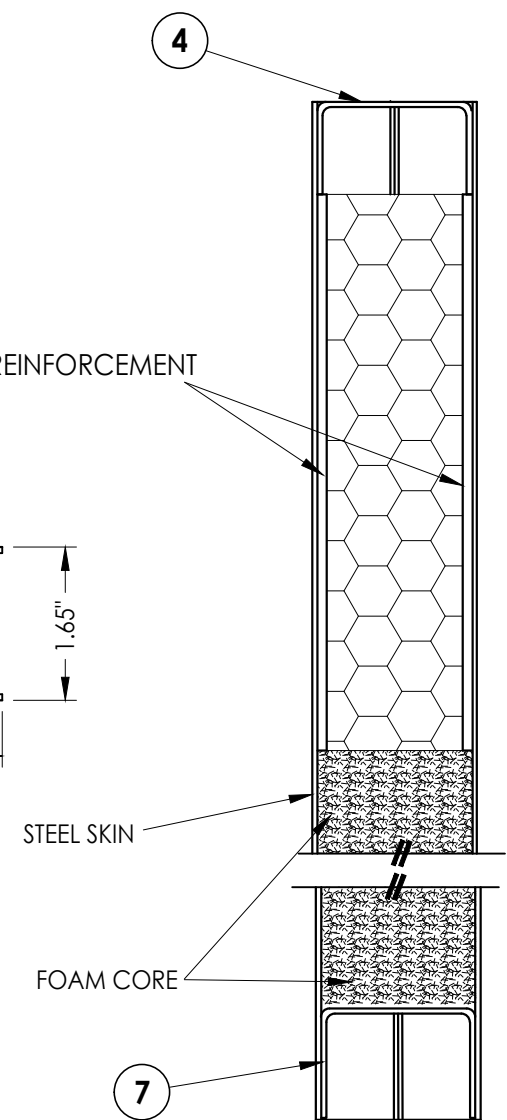
2 4 VERTICAL CROSS SECTION
