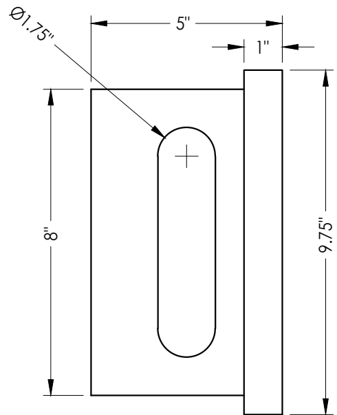
5 LOCK BOX REINFORCEMENT Steel
